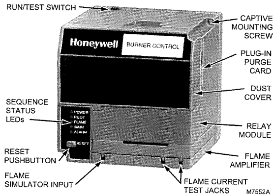
Fig. 1. Relay Module and sequence status LEDs.
